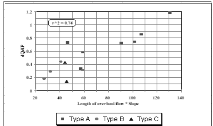
Figure 6 Relation of dQ/dP to the transfer function S * L_{of}
