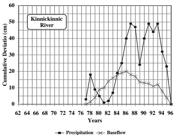
Figure 4 Type C watershed responses. Both sites are urbanized and have cumulative baseflow deviations which exhibit little relation to changes in precipitation.
