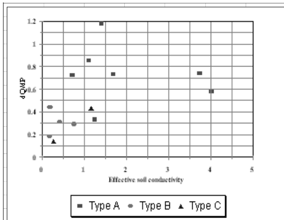
Figure 5 Absence of any obvious relation of dQ/dP to hydraulic conductivity
