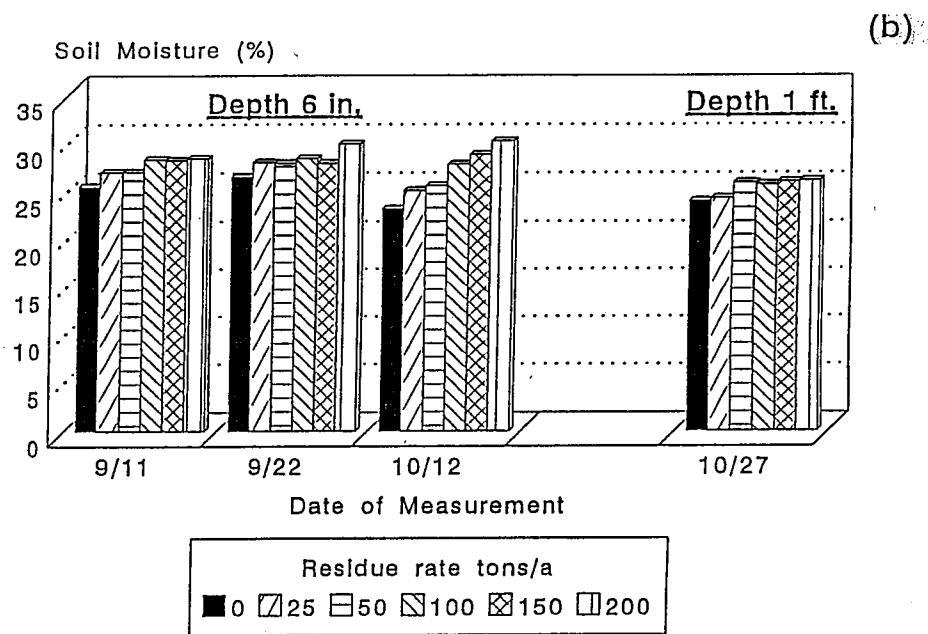
Figure 3. Effect of residue treatments on soil temperature (a) and soil moisture (b), fall 1992.
