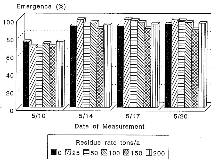
Figure 11. Effect of residue treatments on corn emergence, 1993.
