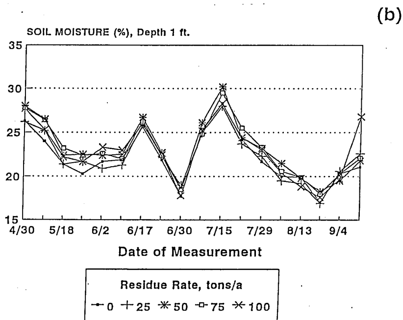
Figure 2. Effect of residue treatments on soil temperature (a) and soil moisture (b), spring and summer 1992.
