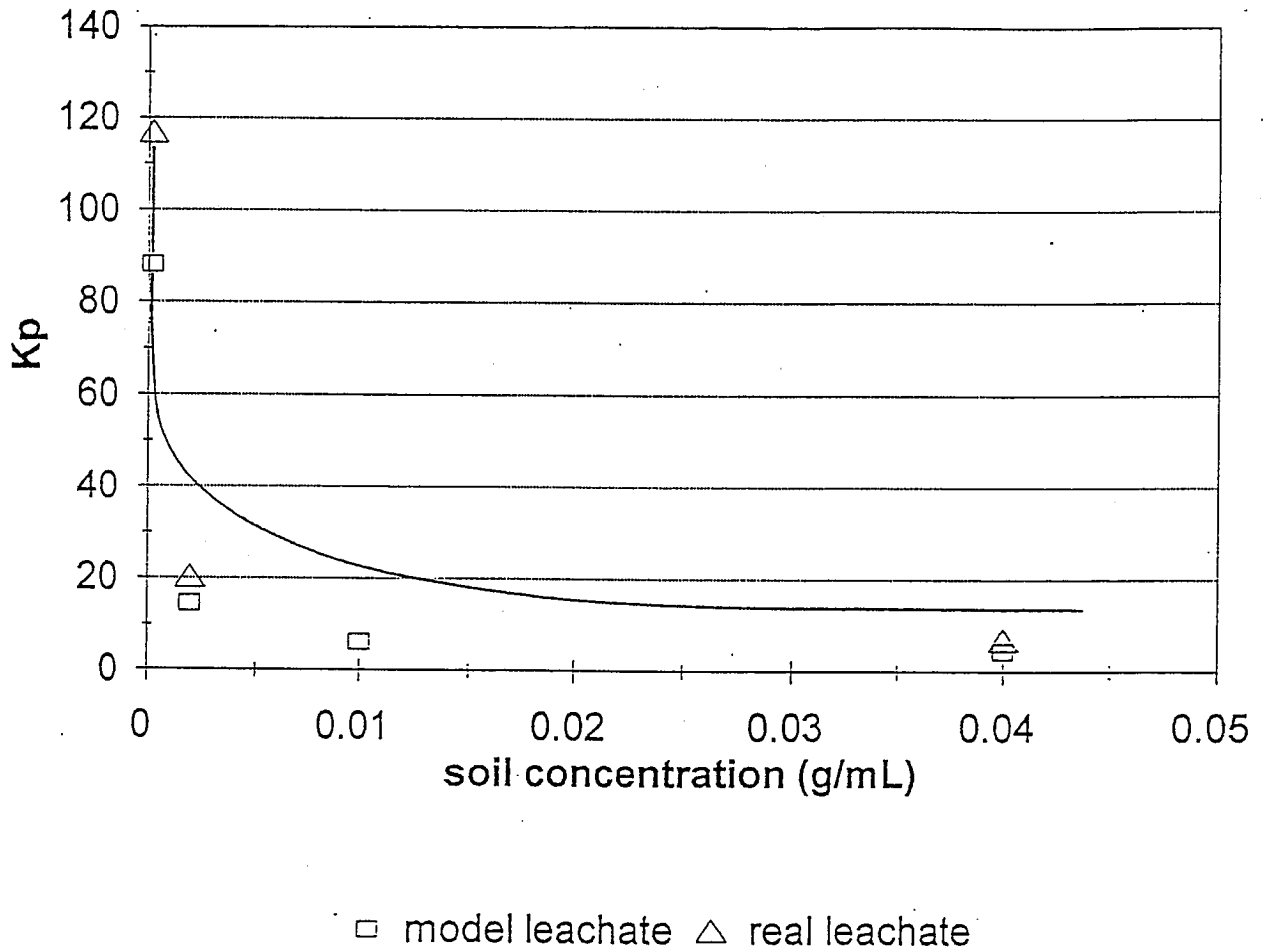
Figure 3. Sorption coefficients of naphthalene vs. soil concentration plotted at a constant leachate concentration of 250 ppm. Squares represent model leachate; triangles represent real leachate. The solid line is the modeled best fit.
