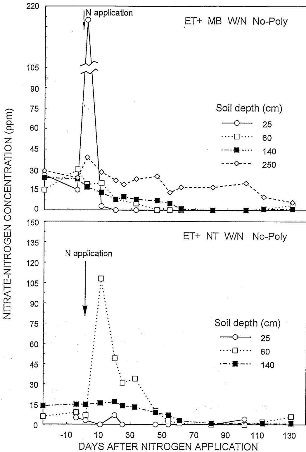
Figure 5. Soil solution NO 3 -N concentrations (average of three treatment replications) for ET+, MB (A) and NT (B) no-polymer treatments LWVR-Arena project, 1990.
