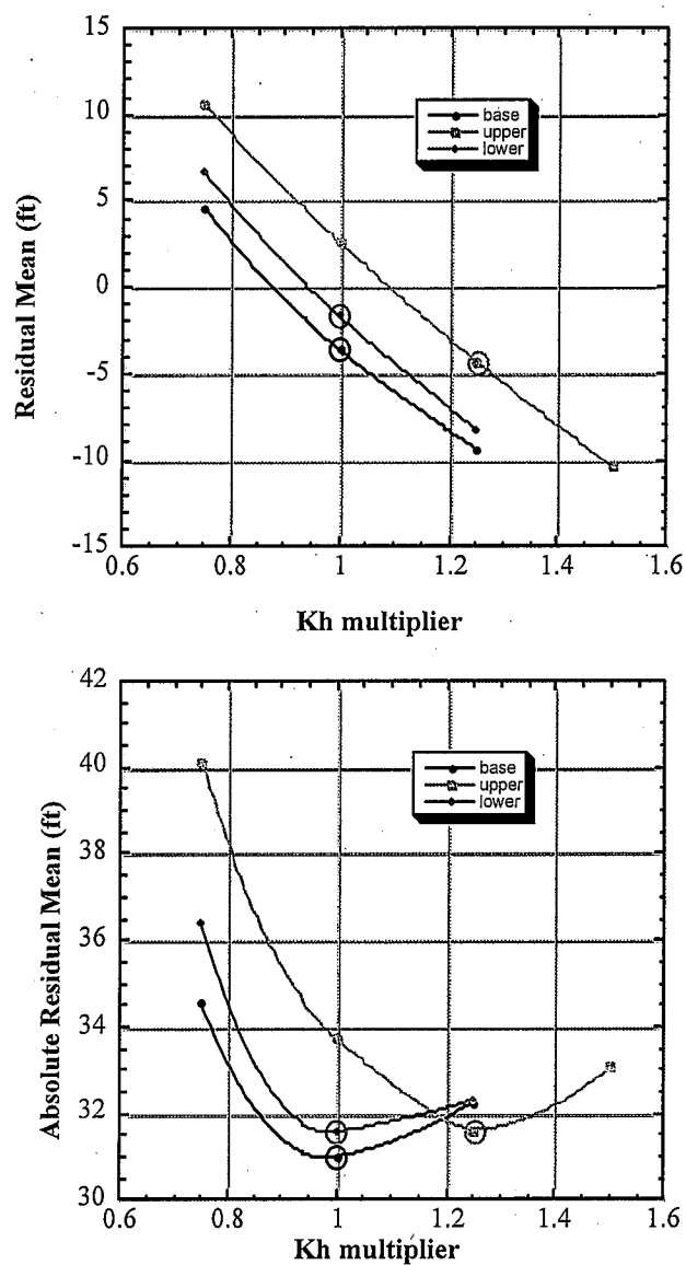
Figure 27. Calibration statistics for the different pumping estimates. The sandstone multipliers for the final calibrated models are circled (no change, a value of 1, for the base and lower estimates, a value of 1.25 for the upper estimate).
