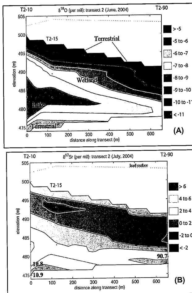
Figure 4. Transect 2. (A) Contours of \delta^{18}\text{O} in cross section, June 2004. (B) Contours of \delta^{87}\text{Sr} in cross section, July 2004. Numbers (10.8, 10.9 and 90.7) indicate sampling locations.
