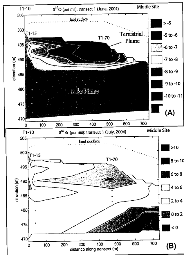
Figure 3. Transect 1. (A) Contours of \delta^{18}\text{O} in cross section, June 2004. (B) Contours of \delta^{87}\text{Sr} in cross section, July 2004.
