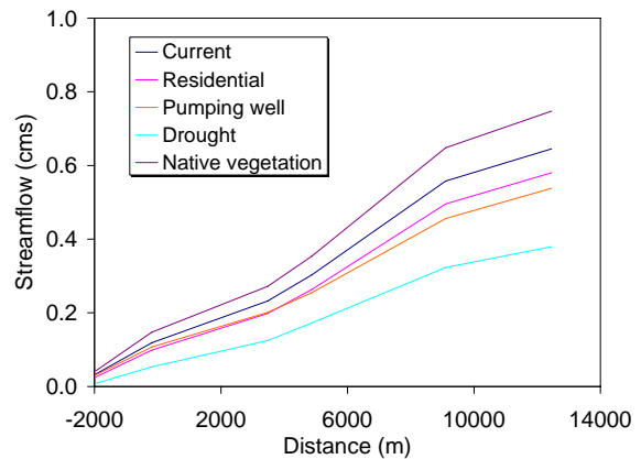
Figure 5. Simulated baseflow of Rowan Creek for different land-cover and climatic conditions.
