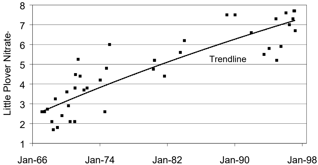
Figure 1. Increasing nitrate-N in Little Plover River baseflow (Albertson and Shaw, 1998).
