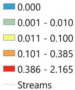
Figure B 26. Imidacloprid concentrations in surface water.
