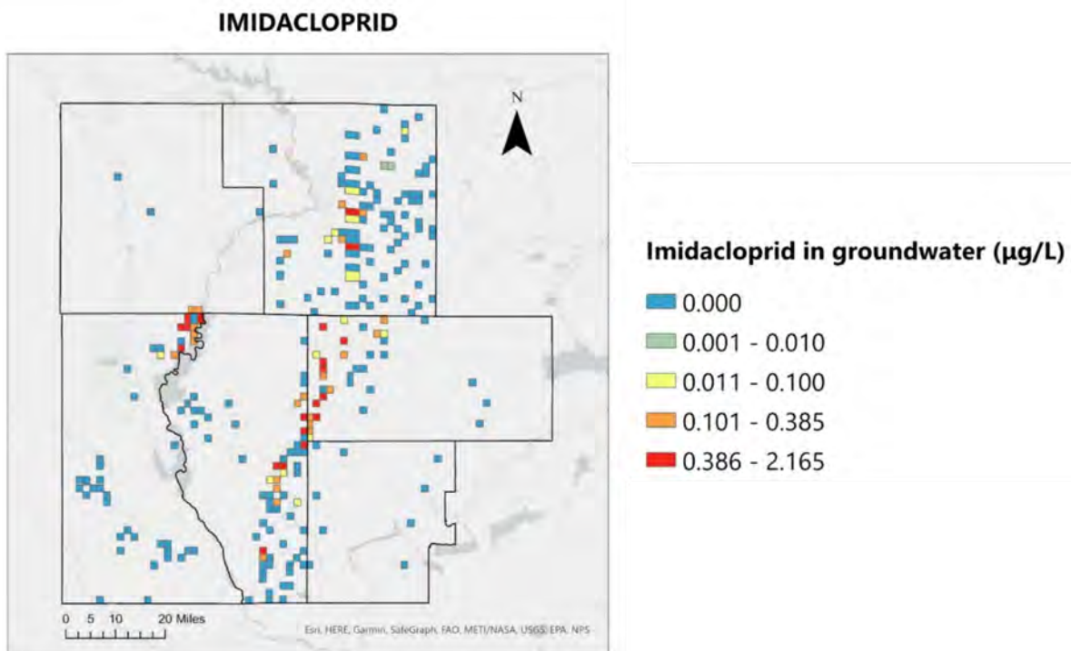
Figure 10. Imidacloprid concentrations in groundwater.
