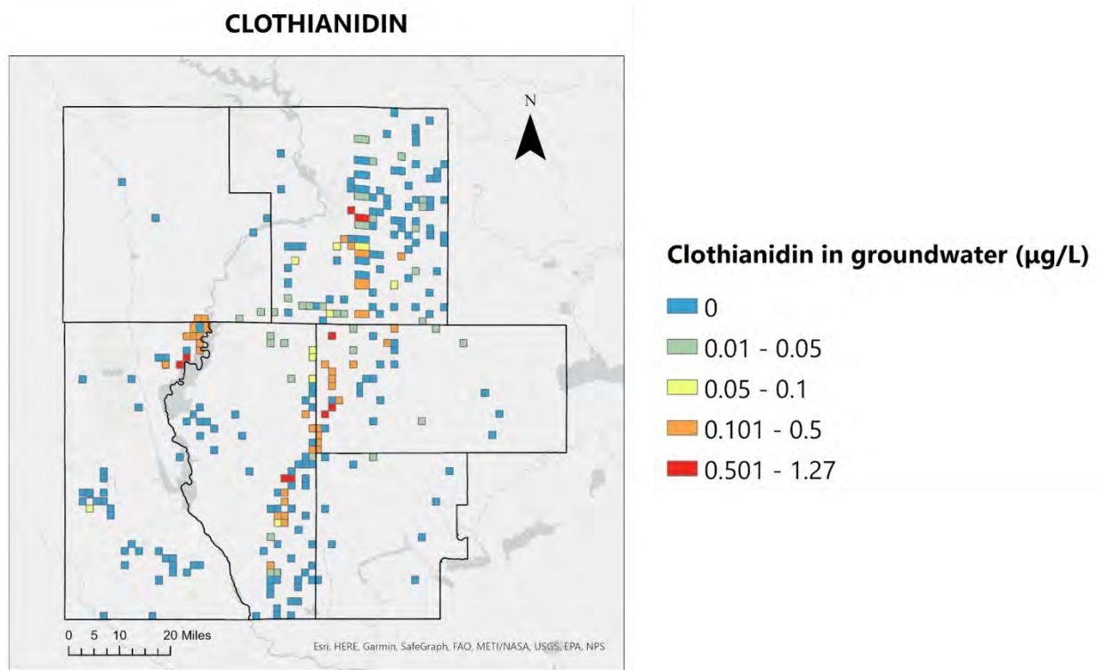
Figure 9. Clothianidin concentrations in groundwater.
